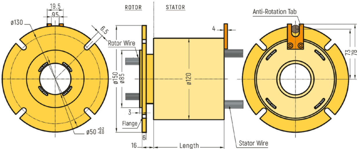
RX-ETH502 - Optional Flange Version (Drawing only exemplary, further details on request)
