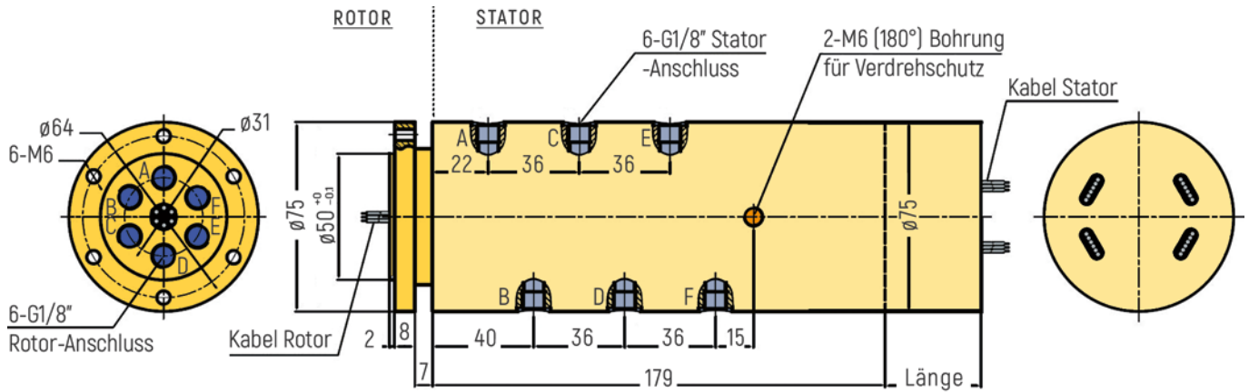
RX-PN1806-QS2-B - G1/8" Anschluss
