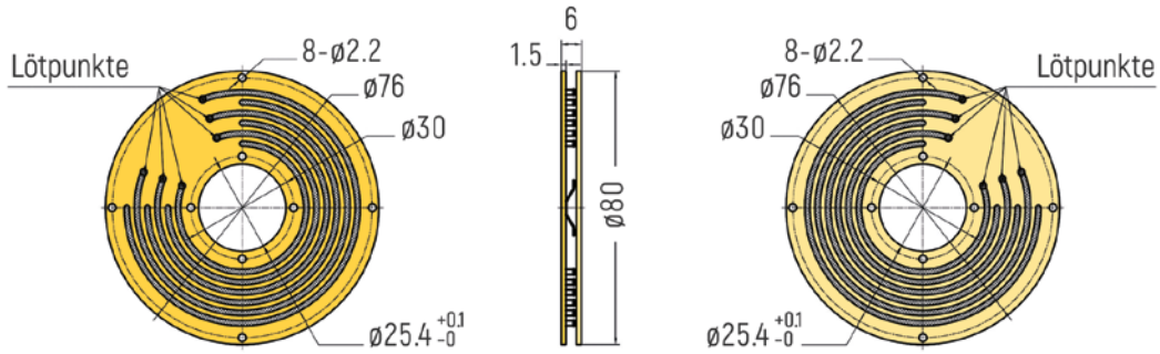
RF-PC2506 - 6 Ringe
