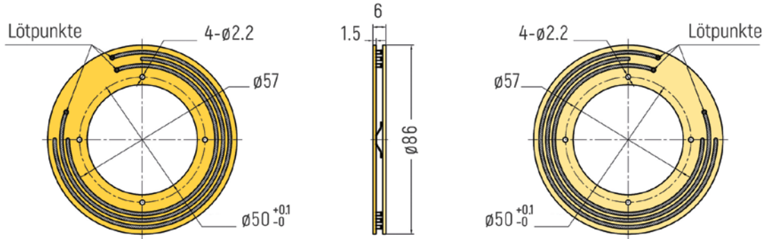
RF-PC5006 - 3 Ringe
