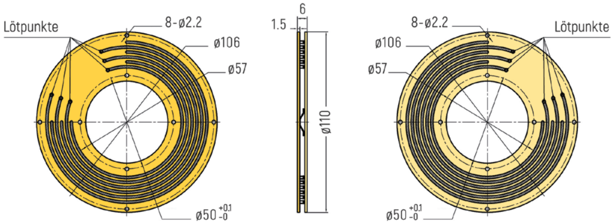
RF-PC5006 - 6 Ringe
