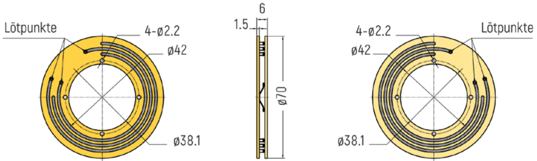
RF-PC3806 - 3 Ringe
