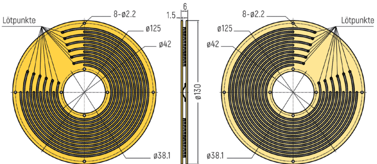
RF-PC3806 - 12 Ringe
