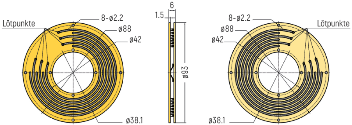
RF-PC3806 - 6 Ringe
