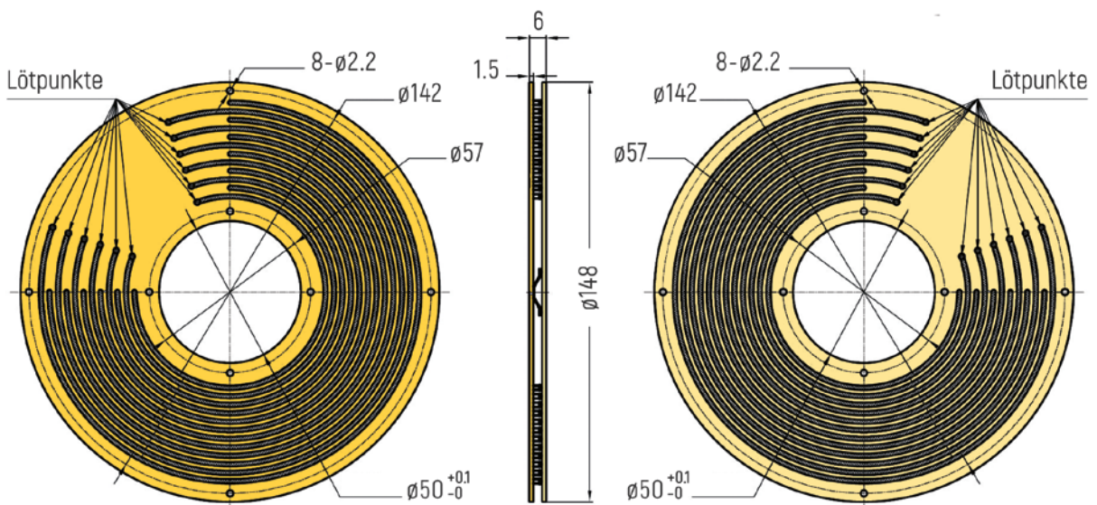
RF-PC5006 - 12 Ringe
